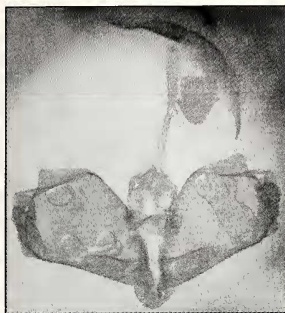
Fig. 15. Male genitalia of Rhodostrophia tyugui , a junior synonym of R. jacularia . Valvae are spread open fully, i.e. pressed flat, unlike in Fig. 7. Juxta is attached to phallus (upper right hand corner) (photo and slide: S. Vasilenko).
